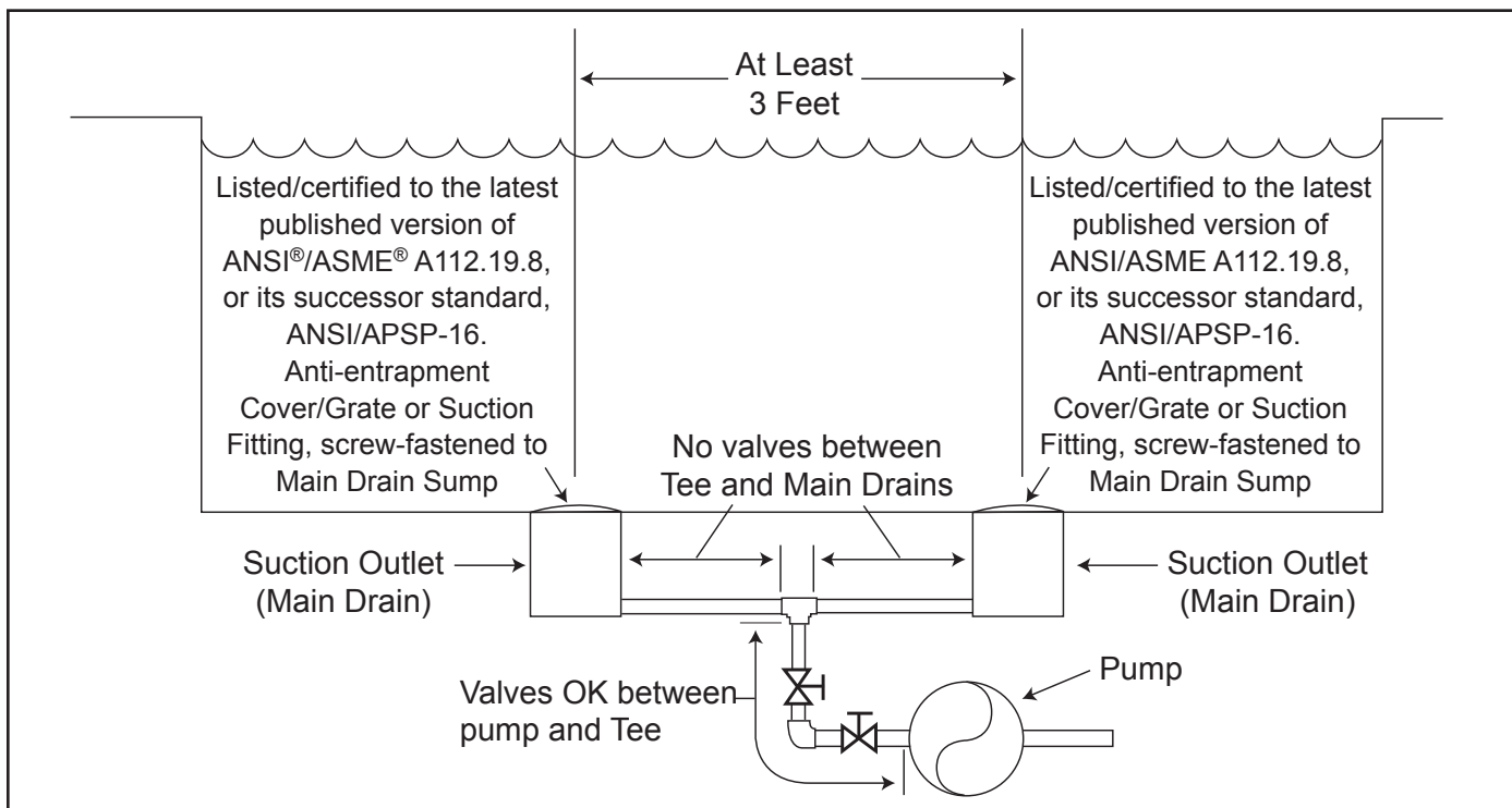
Figure 1. Number of Suction Outlets Per Pump
