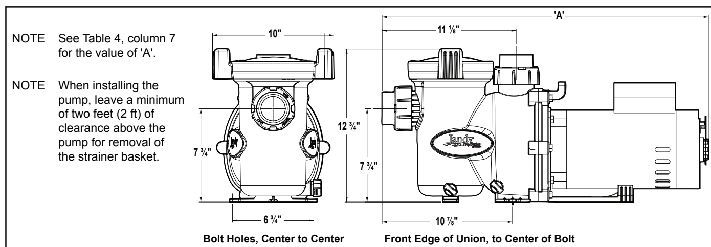
Figure 6. FHP Pump Dimensions (without Base or Spacers)
