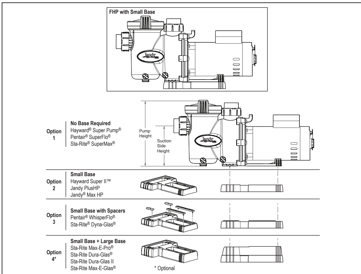
Figure 3. FHP Pump and Base Options
